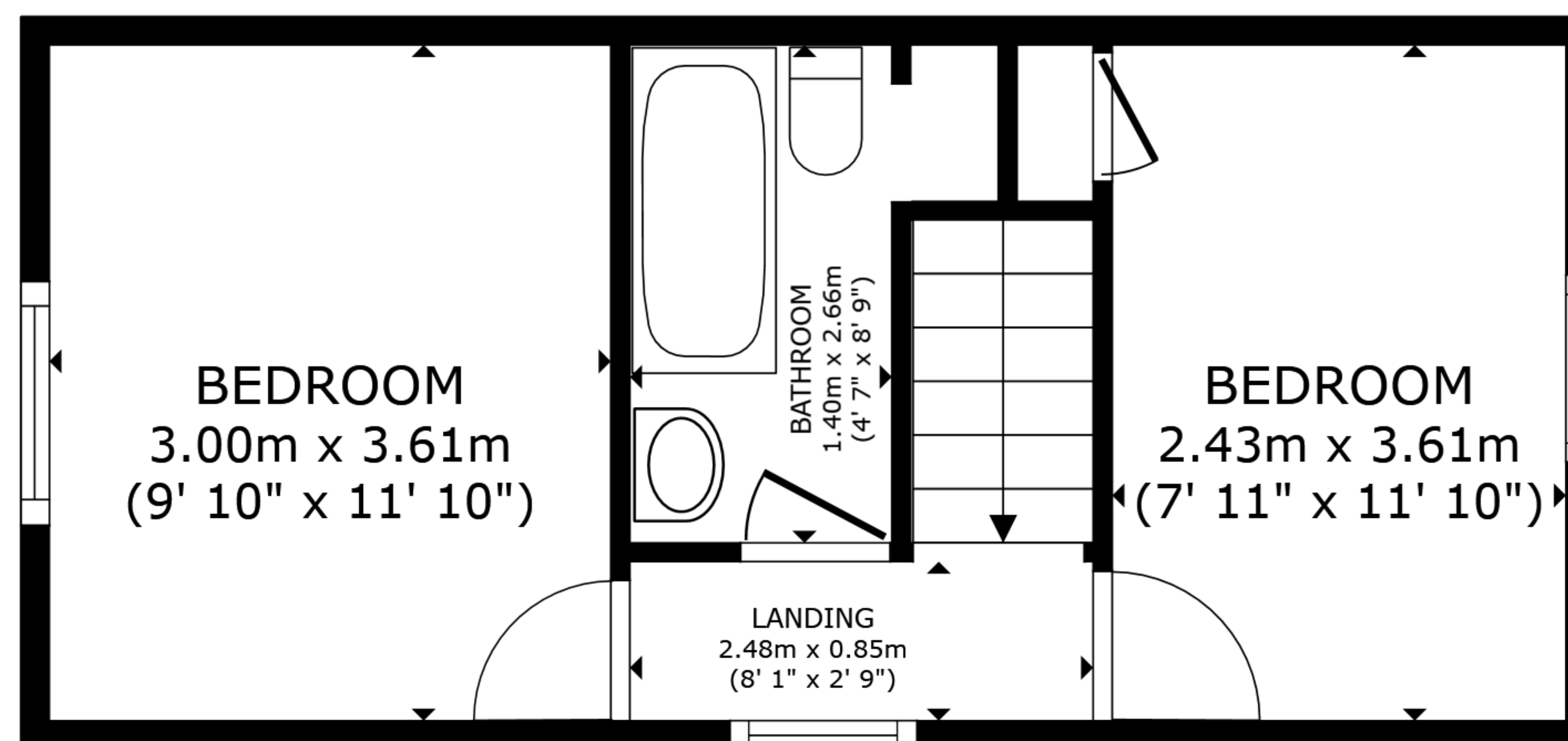
FLOOR 2
